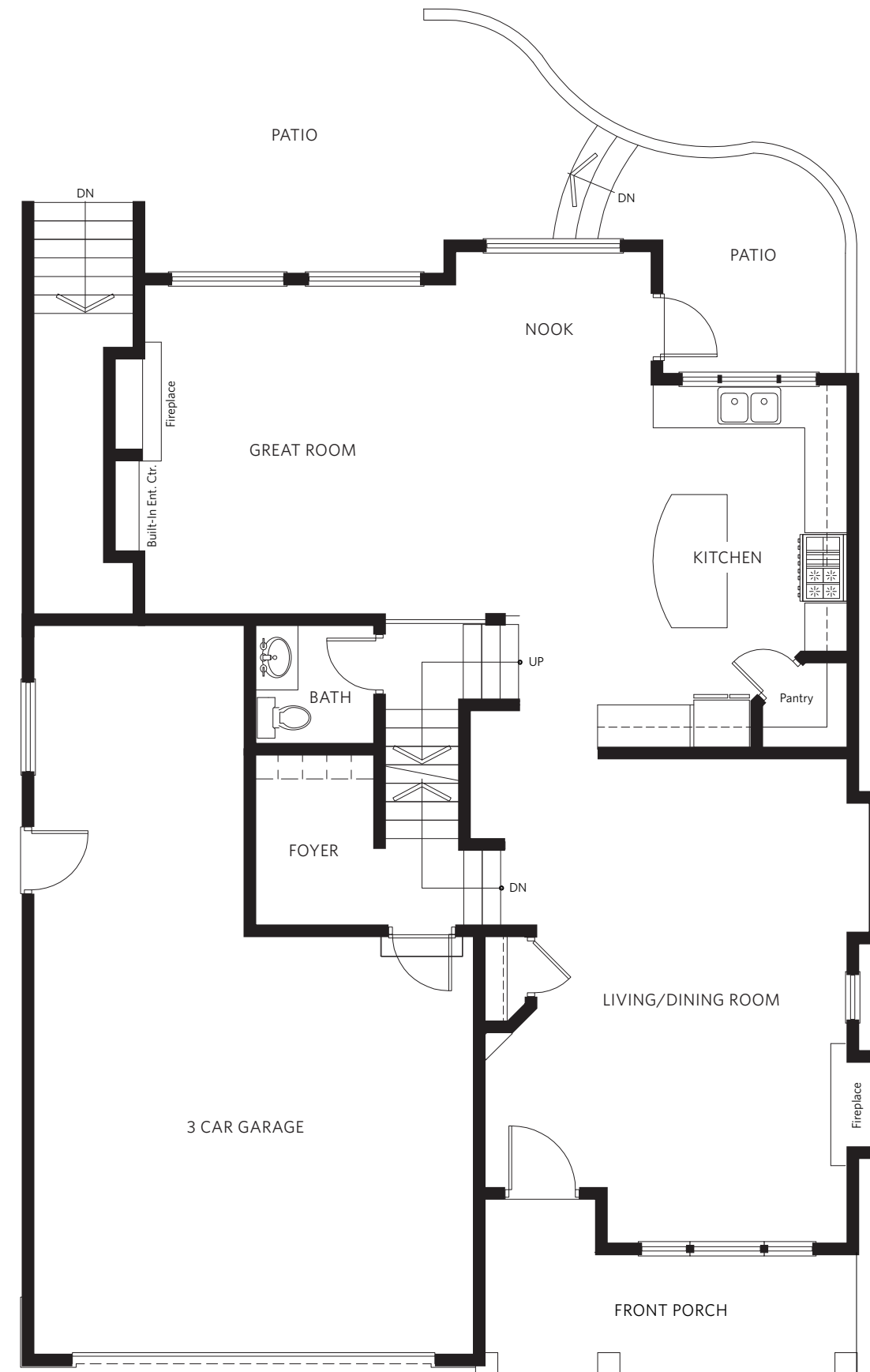
Main Floor Plan - 1082 Sq. Ft. Garage 531 Sq. Ft. W/10' Clearance
